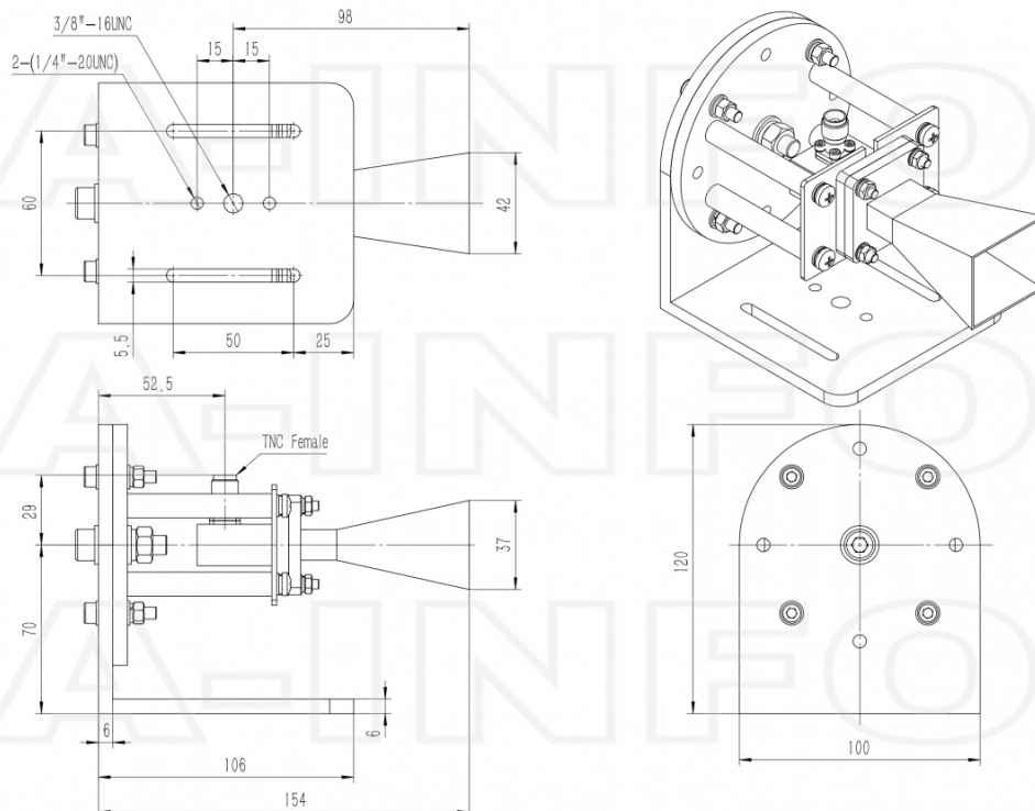
TNC Female Output with L Type Mounting Bracket (Option, P/N: LB-90-10-C-MBL)
