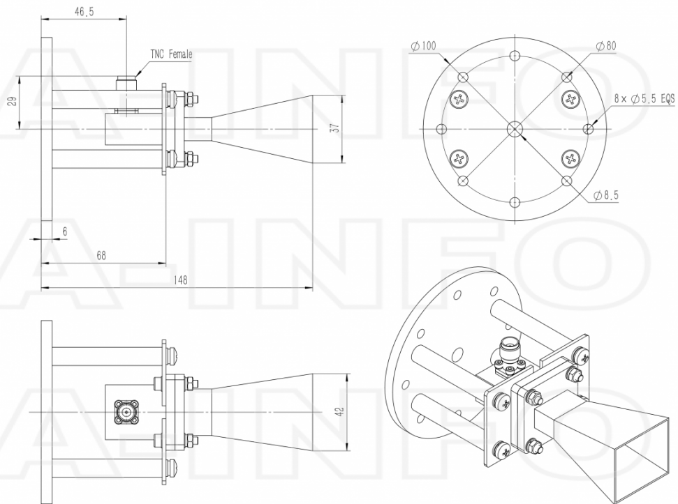
TNC Female Output with Round Mounting Bracket (Option, P/N: LB-90-10-C-MB)
