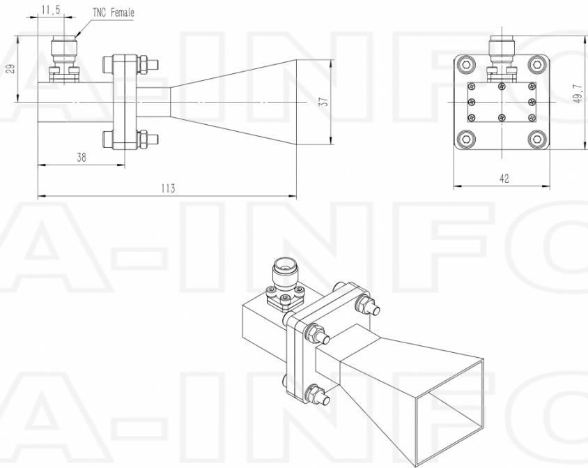
TNC Female Output (P/N: LB-90-10-C-TF)
